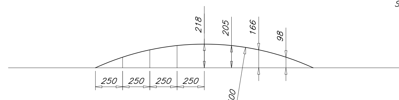
DETAIL C-6 CABIN TOP CAMBER
