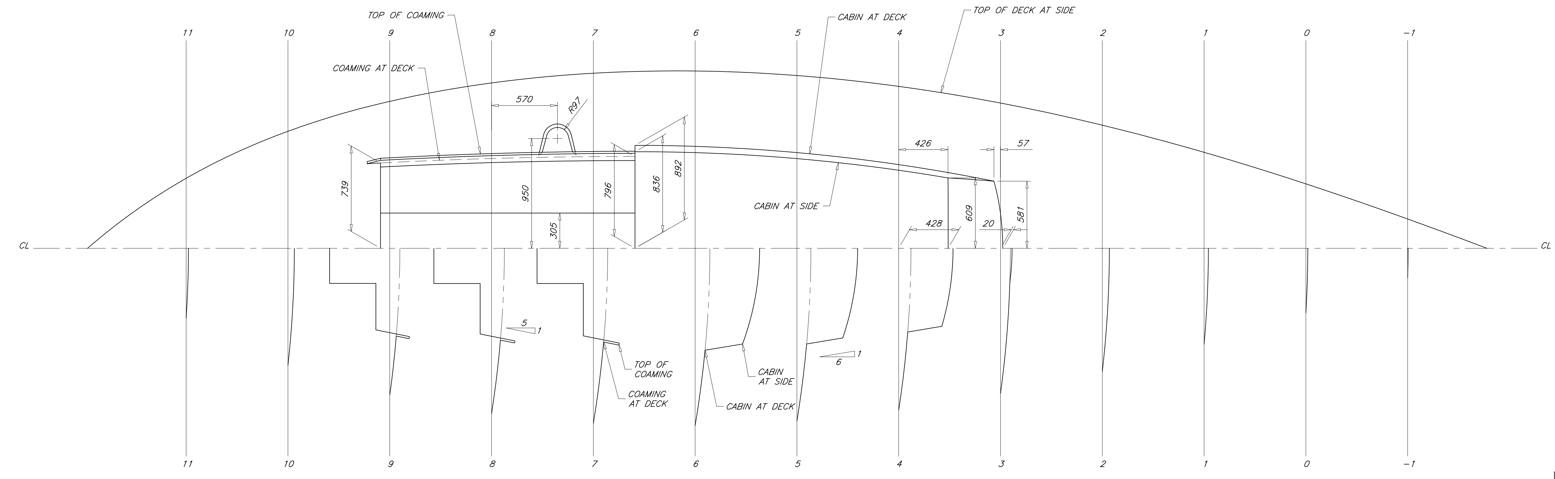
PLAN A-5 STATION SECTIONS
