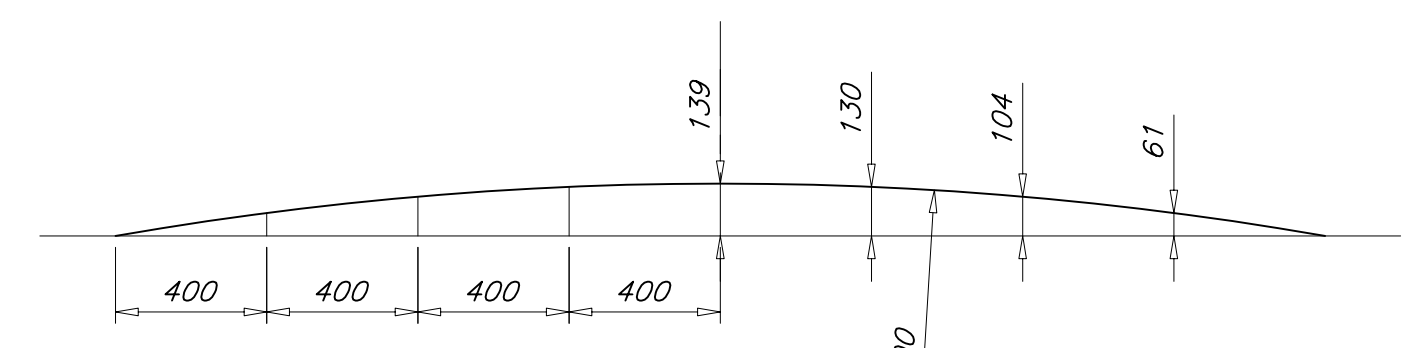
DETAIL C-3 DECK CAMBER
